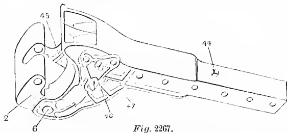
Fig. 2267. Perspective View of Underside.
